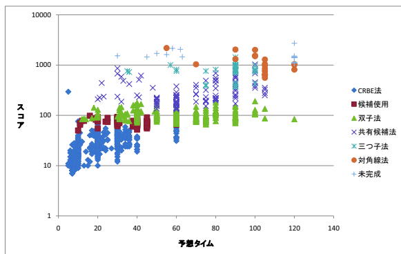
図 28 予想タイムとスコアの関係. Fig. 28 D -Score and expected solving time by puzzle makers.
