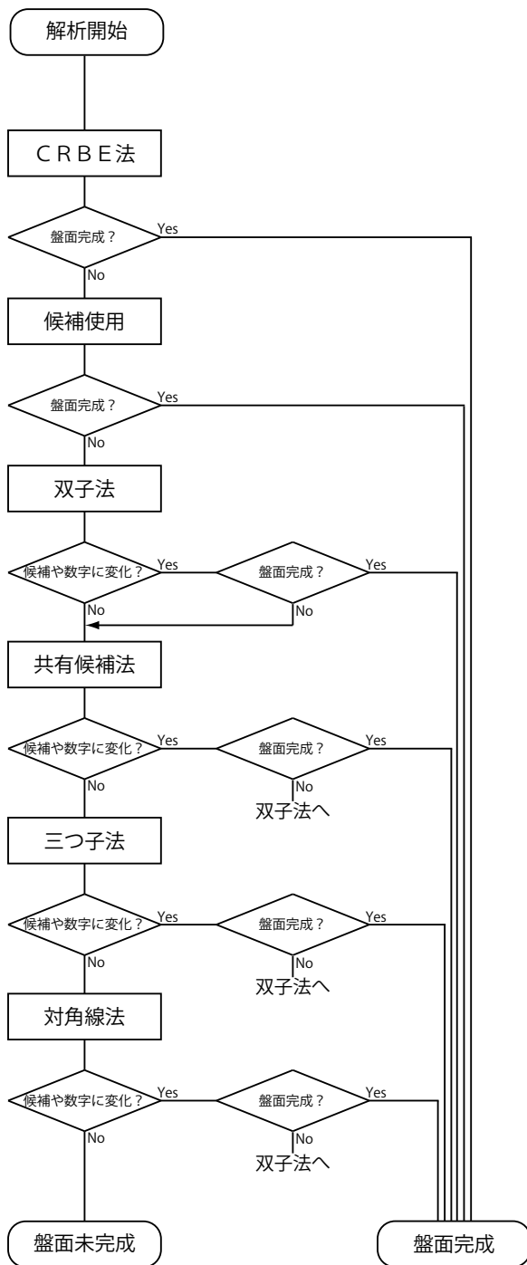
図 25 解法使用順のフローチャート。 Fig.25 Flowchart of the solver using the concluded order of the logics.
