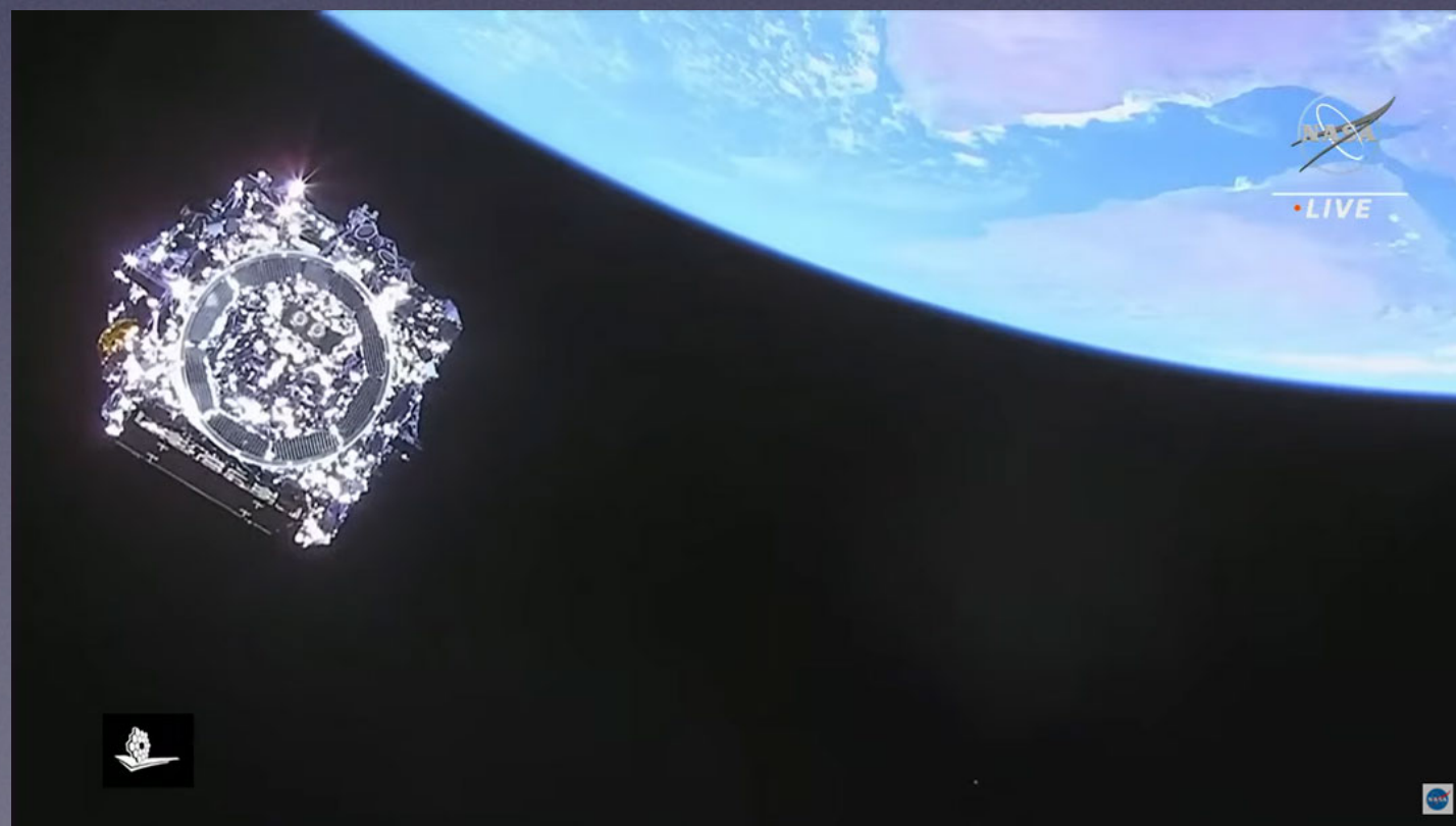
James Webb Space Telescope over Earth 2021/Dec 26
